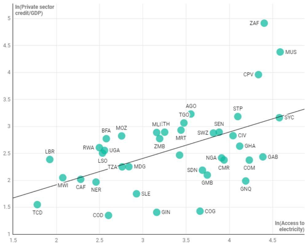
Figure 2: Private sector credit/GDP vs. Access to electricity
